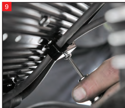
Use the included bolt to hold the bracket to the firewall plate.
