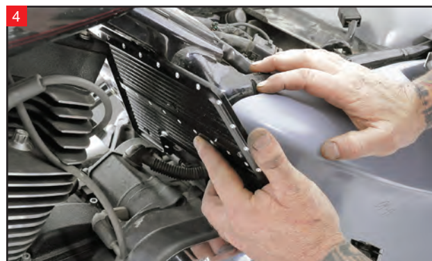
Position the Firewall Plate on the frame, aligning the holes in the frame with the holes in the frame's firewall.
